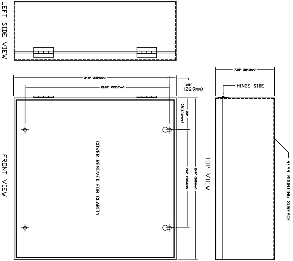
BV5-S3 NEMA 1 ENCLOSURE: Standard Mounting Hole Locations
